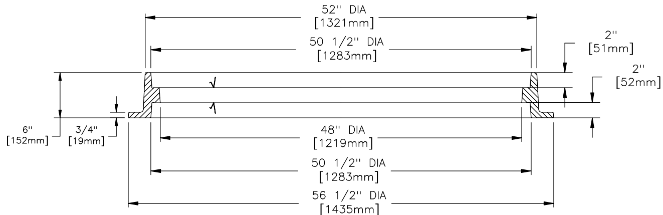
RING SECTION
